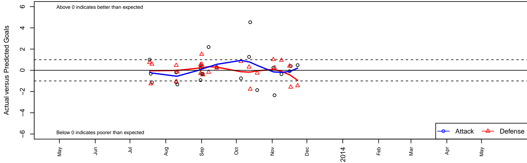
Davis Legacy Millennium G99 Dots are actual minus expected GF (blue circles) and GA (red triangles). Blue line is smoothed change in attack strength. Red is smoothed change in defense strength.
